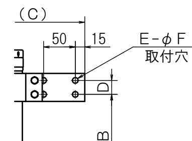
ETC45, 60, 90BJW
